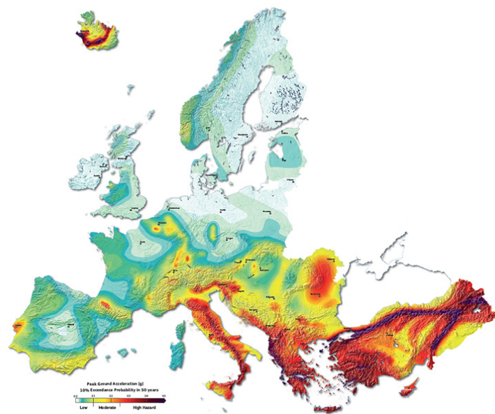
Figure 4. European seismic hazard model (ESHM13) results of peak ground acceleration (PGA) for a 475 year return period and a reference rock condition of Eurocode 8 type A ( V_{s30} = 800\text{m/s} )
