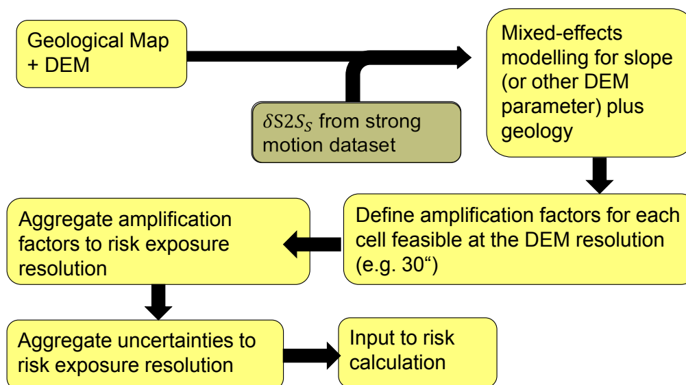
Figure 6. Flowchart showing how the amplification factors will be calculated on the same grid as the exposure model, regardless of the resolution of the proxy data
