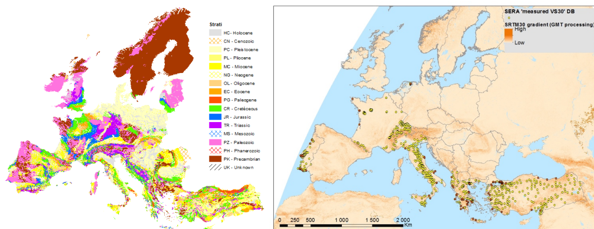
Figure 5. Proxy datasets of simplified stratigraphic map (left) and gradient from the SRTM30 30 arc-second land topography data set, superimposed with measured V_{S30} data (right)
