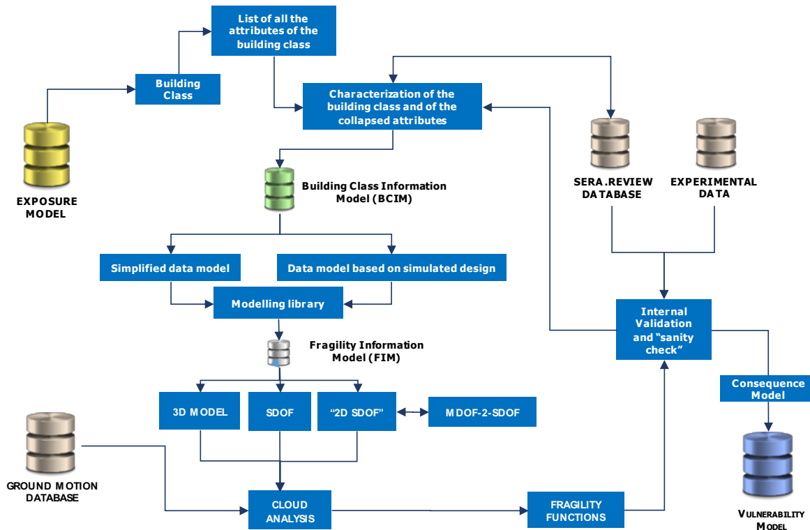
Figure 8. General workflow of the SERA framework for seismic vulnerability analysis
