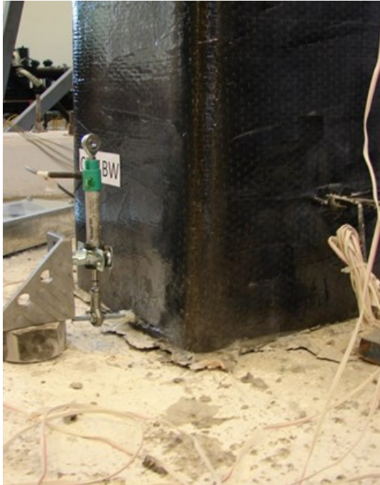
Cracking at column-foundation and column-joint interfaces of the first floor
