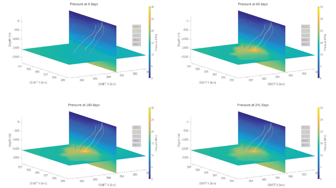
Figure 31: Evolution of the pressure in Húsmúli from the start of reinjection into wells HN9 to HN17
