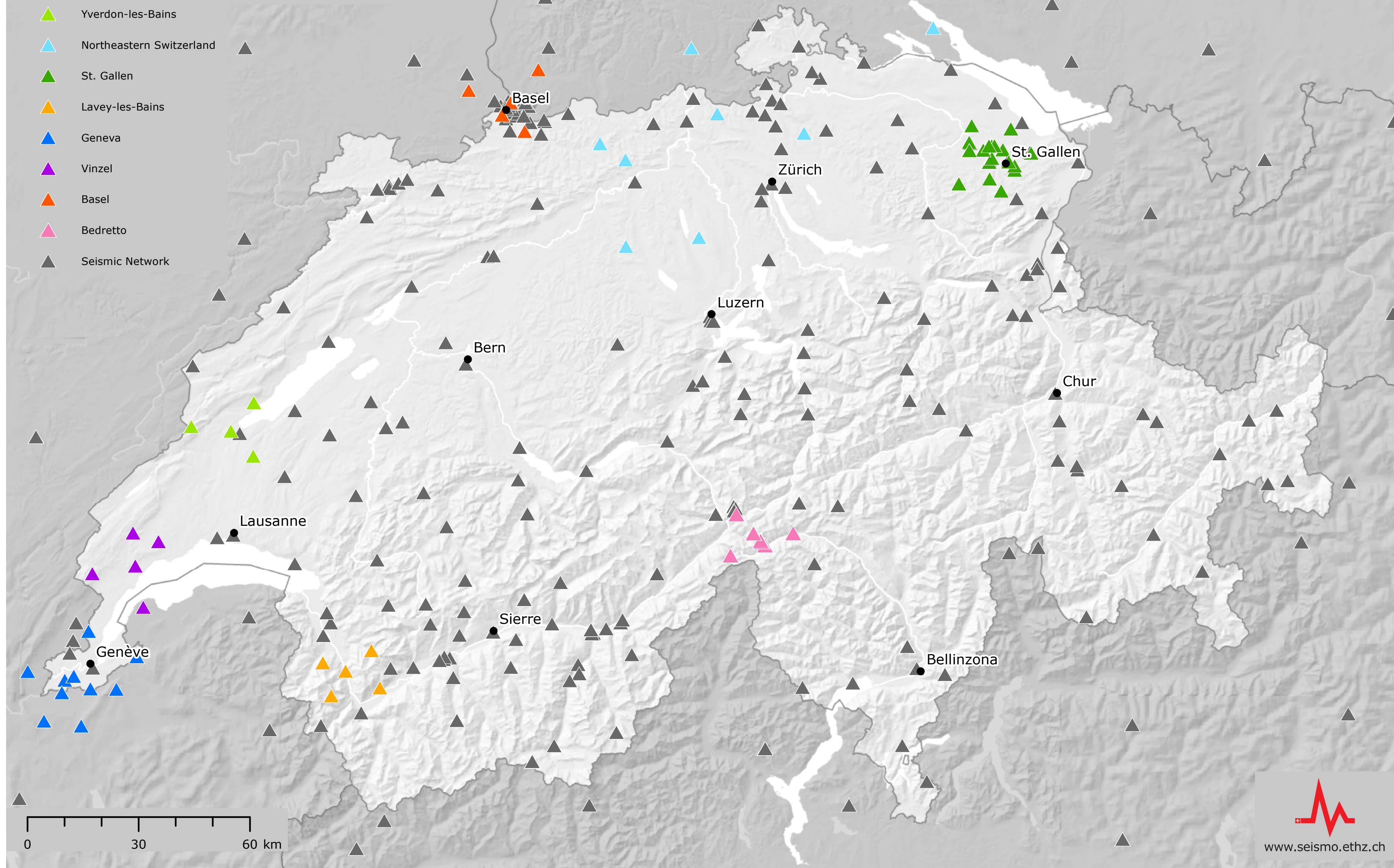
Seismic Network of Switzerland with Special Networks
